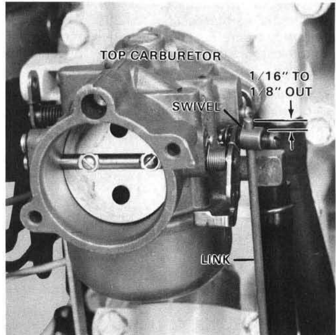
Figure 12. Positioning Choke Link.
