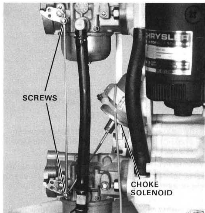
Figure 13. Securing Choke Link.
