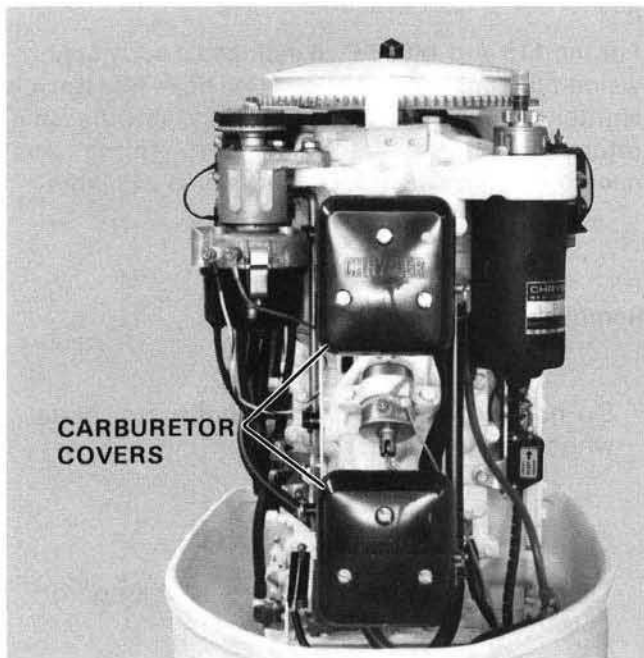
Figure 11. Removing Carburetor Cover.
